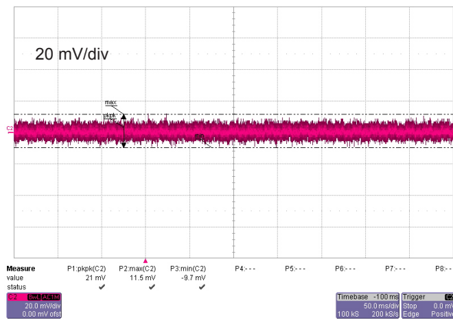
Figure 15: Output noise
