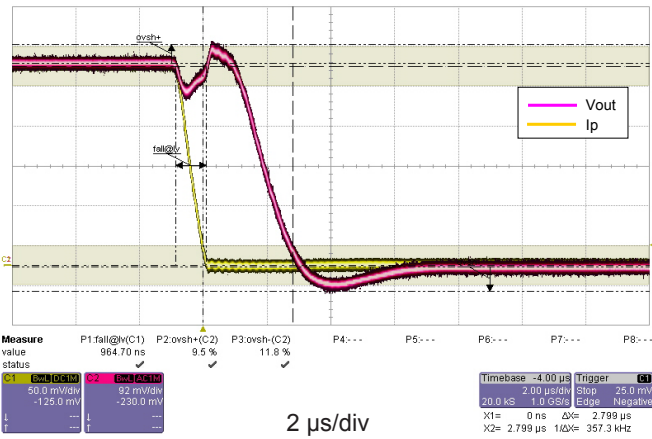
Figure 13: Step response
