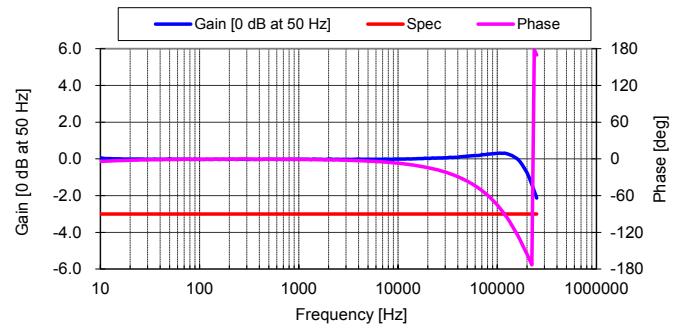
Figure 7: Frequency response
