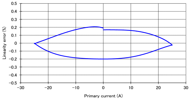
Figure 11: Linearity error
