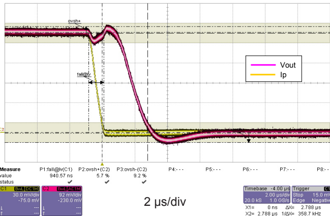
Figure 8: Step response
