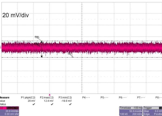
Figure 10: Output noise
