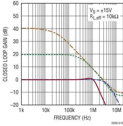
Closed Loop Gain vs Frequency
